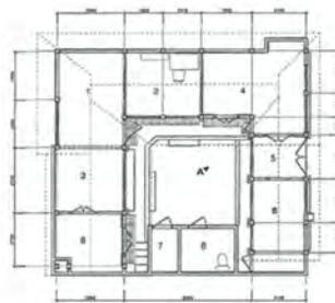
삼청동 35-129 (안방 : 2,680mm, 사랑방 : 1,830mm)
